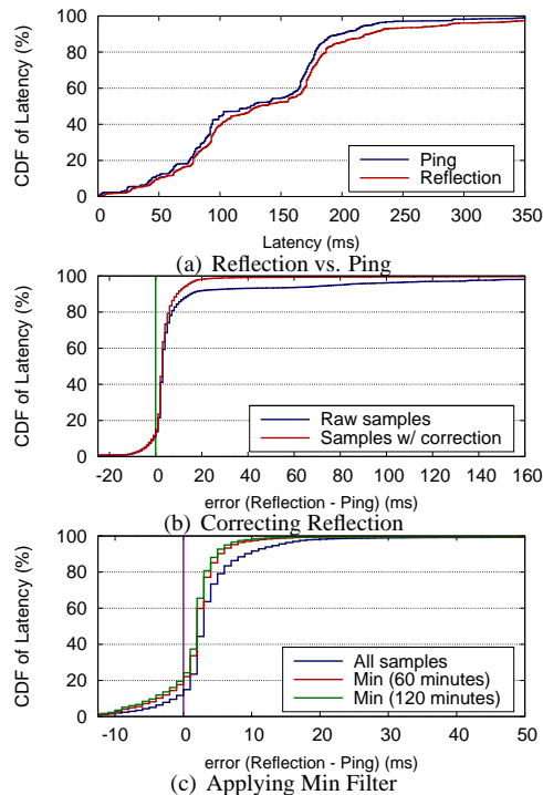
Figure 3: Latency Comparison
