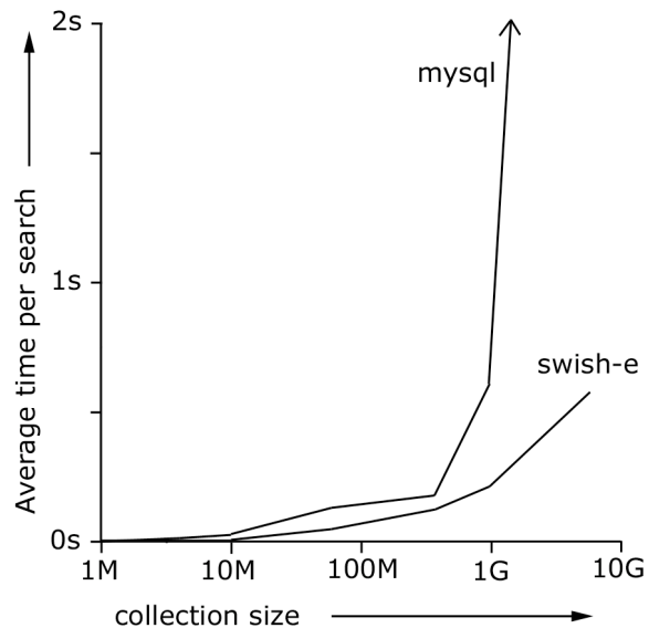
Graph 1: MySQL against swish-e, showing average search time vs. collection size.
